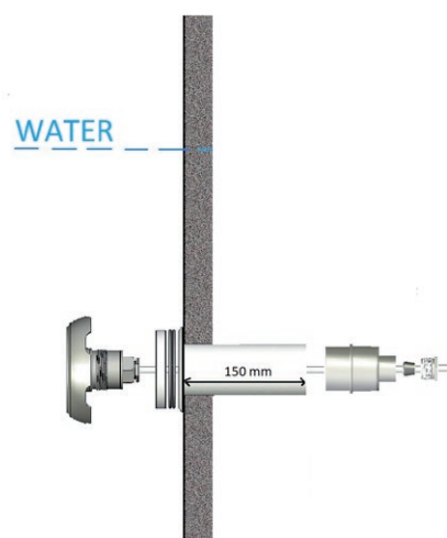
Above ground pool
