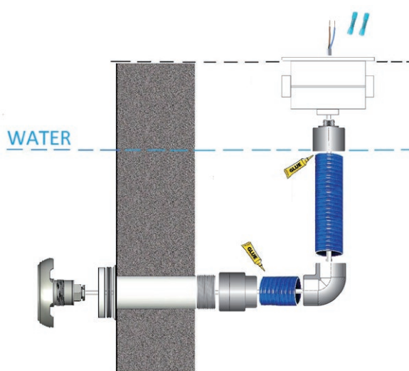
Inground pool with liner
