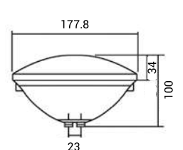
Bulbs (Dimensions in mm)
